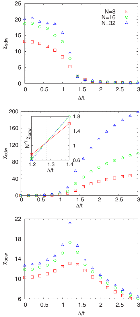
FIG. 1. (Color online) Spin density wave (top), charge density wave (middle), and bond ordered wave (bottom) susceptibilities versus staggered site energy \Delta for U=6t , V=1.5t , \beta t=8 , and N=8, 16, 32 . The SDW-CDW transition occurs at close to the t=0 value, \Delta=U/2-V . BOW correlations are enhanced in the intermediate region. In the inset to the middle panel, the scaled \chi_{\text{CDW}} is shown for \gamma=1 . The scaled susceptibilities cross at \Delta_c/t=1.278 , indicated by the vertical dotted line.
