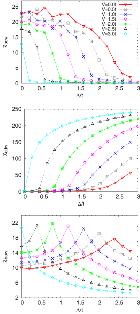
FIG. 3. (Color online) Spin density wave (top), charge density wave (middle), and bond ordered wave (bottom) susceptibilities versus staggered site energy \Delta for U=6t , V=0.0t , (0.5t) , 3.0t , and N=32 .
