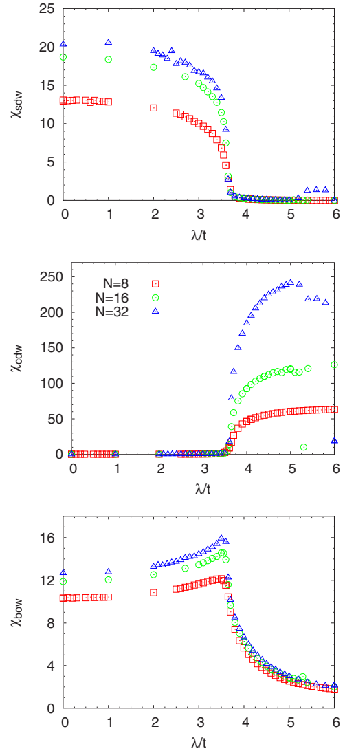
FIG. 6. (Color online) Spin density wave (top), charge density wave (middle), and bond ordered wave (bottom) susceptibilities versus electron-phonon coupling \lambda for U=6t , V=1.5t , \omega_0=2t , \beta t=8 , and N=8, 16, 32 .
