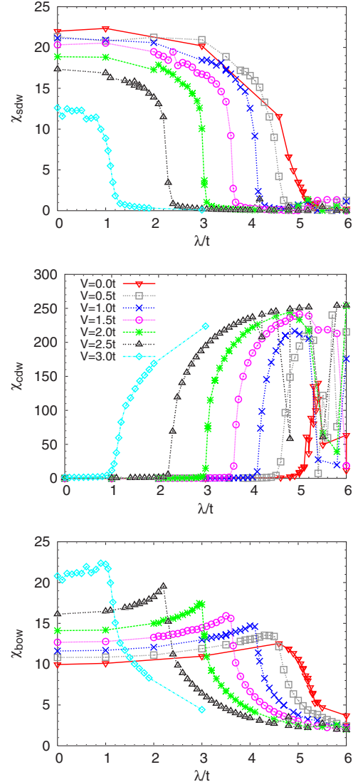
FIG. 7. (Color online) Spin density wave (top), charge density wave (middle), and bond ordered wave (bottom) susceptibilities versus electron-phonon coupling \lambda for U=6t , V=0.0t ( 0.5t ), 3.0t , \omega_0=2t , and N=32 .
