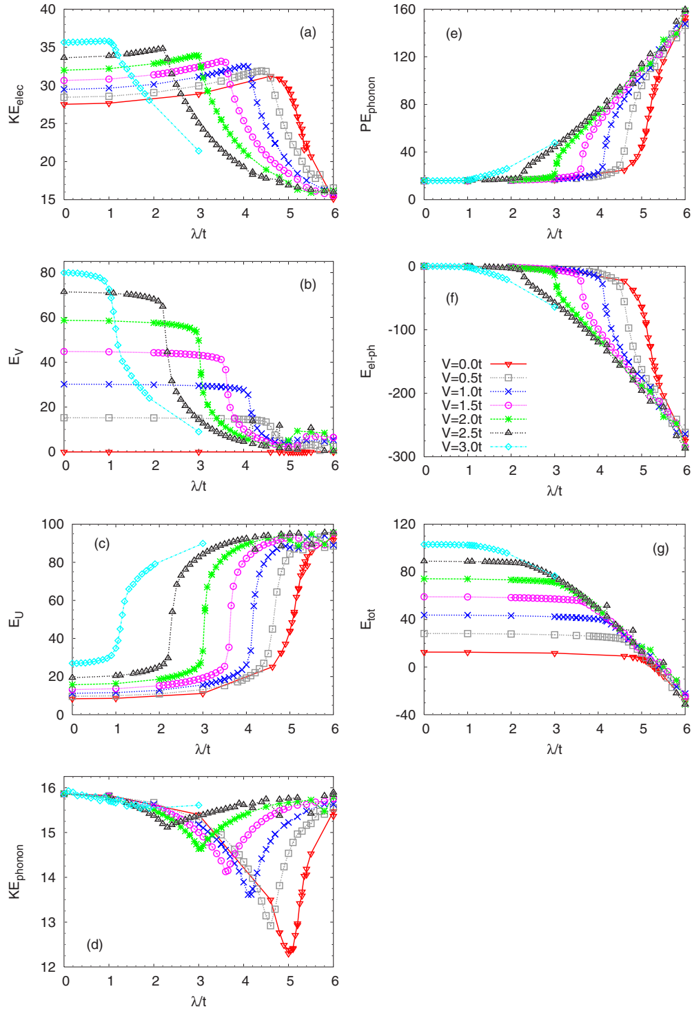
FIG. 8. (Color online) (a) Kinetic (hopping), (b) intersite Coulomb, (c) on-site Coulomb, (d) kinetic (phonon), (e) potential (phonon), (f) electron-phonon coupling, and (g) total energies versus coupling constant \lambda for U=6t , V=0.0t ( 0.5t ), 3.0t , \beta t=8 , \omega_0=2t , and N=32 . The fluctuations in the phonon kinetic energy are significantly smaller than those for all other energies for these parameters.
