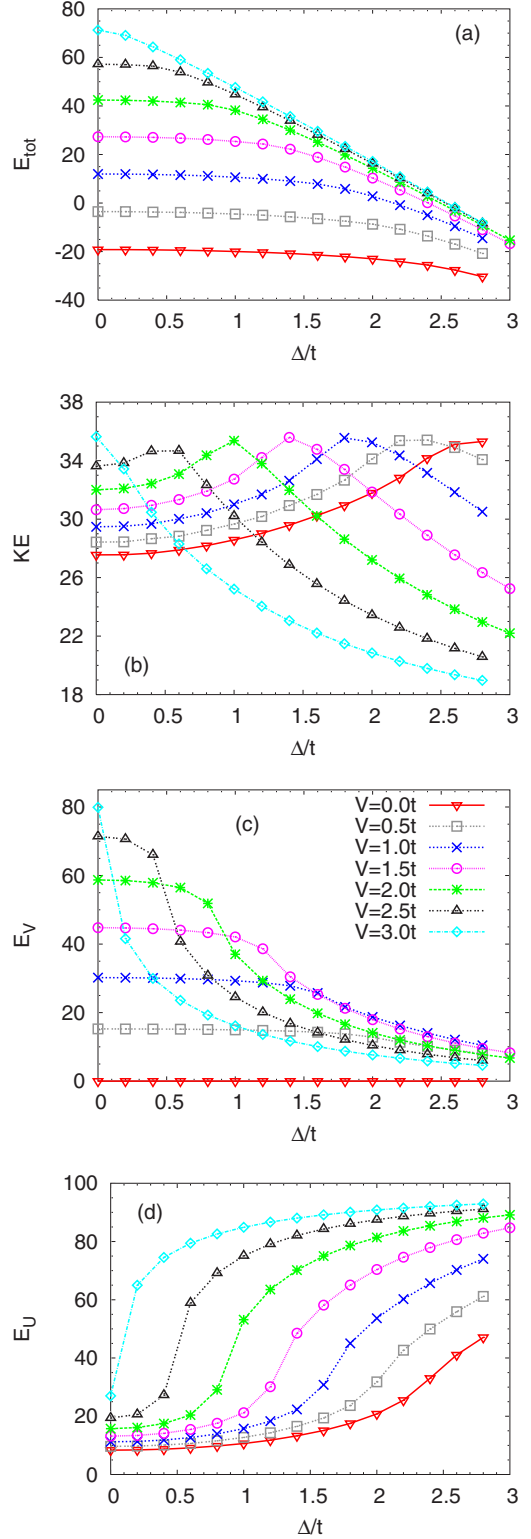
FIG. 4. (Color online) Total (a), kinetic (b), intersite Coulomb (c), and on-site Coulomb (d) energies at fixed U=6t and different V . The inverse temperature is fixed at \beta t=8 and the lattice size at N=32 . The kinetic energy is largest in the region where there is a balance between the CDW and SDW insulating tendencies, in good correspondence with the behavior of \chi_{\text{BOW}} . The intersite interaction energy falls abruptly on entry to the CDW state, and the on-site energies rise steeply as the pairs form.
