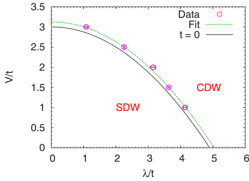
FIG. 9. (Color online) This figure shows the phase diagram for intersite V and electron-phonon coupling \lambda with U=6t , \omega_0=2t , and \beta t=8 . Line with symbols is the result of the WLQMC simulations in this paper. The functional form of the fit is V=a\lambda^2+b . We show the exact result (line without symbols) for the t=0 phase.
