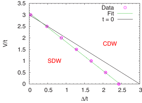
FIG. 5. (Color online) Phase diagram in the intersite V and staggered site energy \Delta plane, with U=6t and \beta t=8 . Line with symbols is the result of the WLQMC simulations in this paper. We also show the exact result (line without symbols) for t=0 . As expected, the strong coupling limit works well at large V , but there are significant deviations as V becomes smaller.
